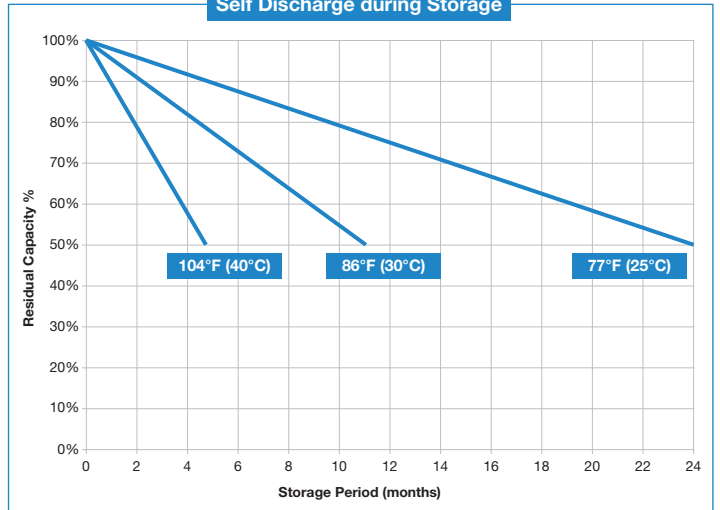
Self Discharge during Storage
