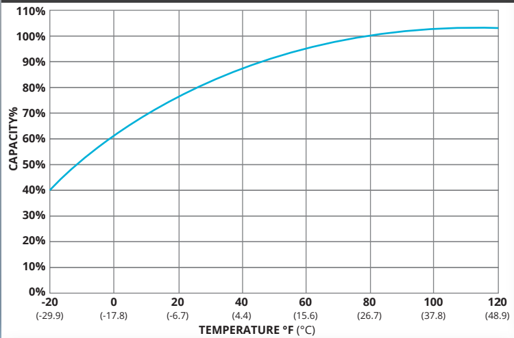
TEMPERATURE vs CAPACITY
