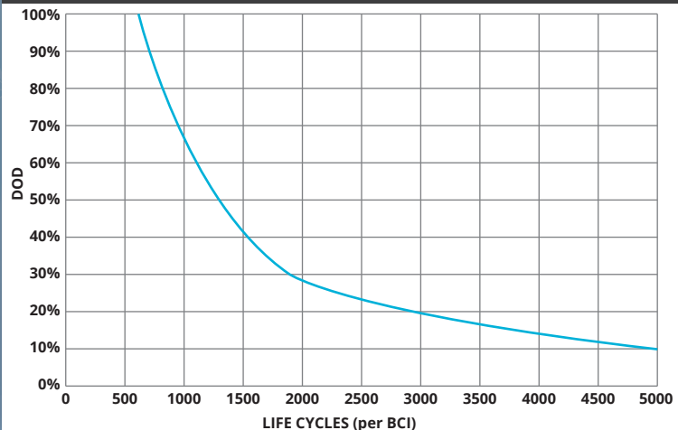
CYCLE LIFE vs DEPTH of DISCHARGE (DOD)
