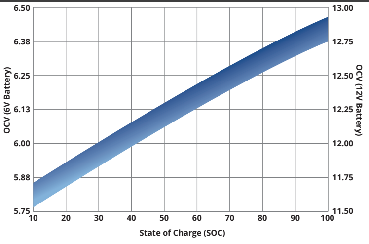
STATE of CHARGE (SOC) vs OPEN CIRCUIT VOLTAGE (OCV)
