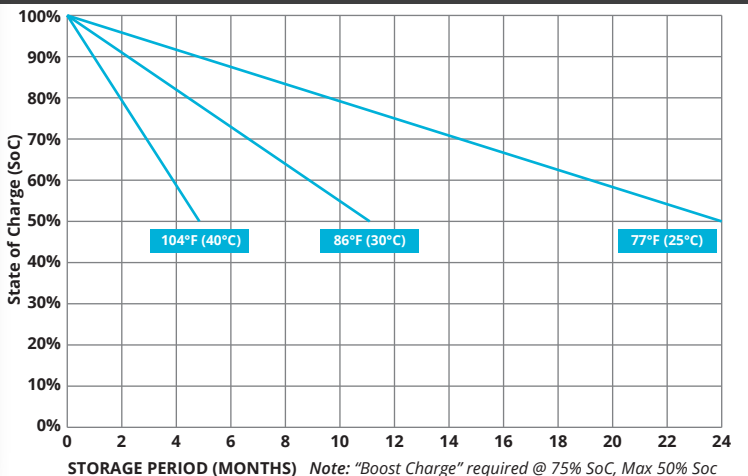
SELF DISCHARGE vs TIME/TEMPERATURE
